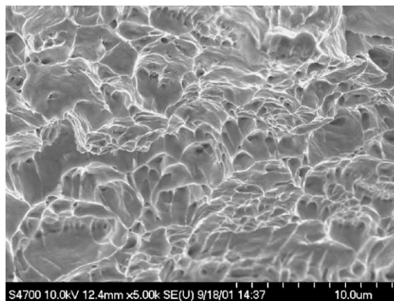
Fig. 6. Fracture surface of a room-temperature-tested tensile specimen from the B1 test after \approx 1 year of exposure. The surface consists of dimples and microvoids, indicating that fracture is ductile.
