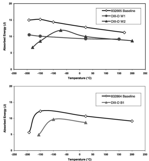
Fig. 3. Charpy impact properties of Heats 832665 and 832864 of V-4Cr-4Ti alloys as affected by exposure to DIII-D environment.
