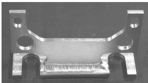
Fig. 1. Baffle support brackets made with a V-4Cr-4Ti alloy for the DIII-D upper radiative divertor.
