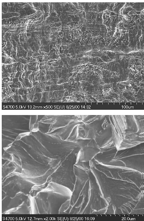
Fig. 5. Whereas the fracture of the W2 Charpy specimen tested at room temperature is completely ductile (top), that of the -150\text{ }^{\circ}\text{C} specimen contained brittle cleavage features near specimen external surfaces (bottom).
